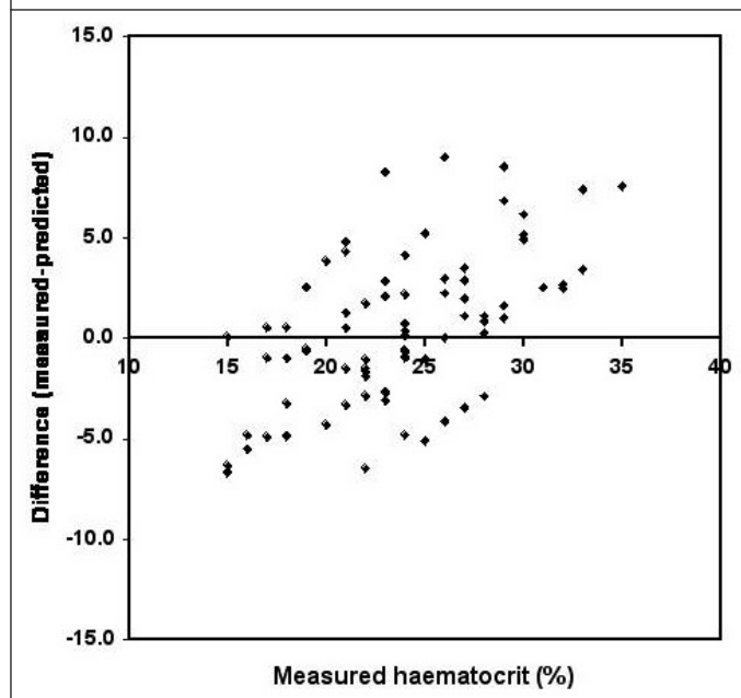
Figure 2: Graph of the differences between measured and predicted haematocrit values during cardiopulmonary bypass on the ordinate versus measured values on the abscissa. The haematocrit values were predicted according to equation-1. There was a tendency to overpredict at low haematocrit values and underpredict at high values. Pearson product-moment correlation coefficient, r = 0.57 , p < 0.001 .
