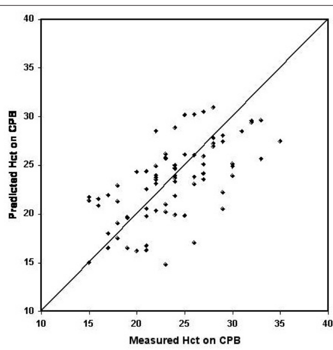
Figure 1: Graph depicting the agreement between measured haematocrit during cardiopulmonary bypass and the haematocrit predicted by equation-1. The diagonal line is the line of identity, which indicates perfect agreement.
