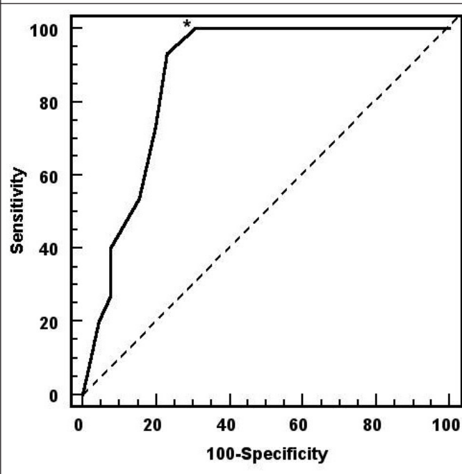
Figure 3: The receiver operating characteristic (ROC) curve for calculated probabilities of obtaining measured haematocrit values of < 20\% during cardiopulmonary bypass. The curve was constructed by calculating the sensitivity and false positive rate ( 100 - \text{specificity} ) for each possible cut-off point for the predicted haematocrit ( Hct_{pred} ) between Hct_{pred} values of 15% and 31% according to equation-1 (see Table 4). The area under the curve is 0.869 (95% confidence interval 0.775 to 0.934). The dotted line of identity indicates 50% prediction probability i.e. the line along which a test has no discriminatory power. The asterisk indicates the selected optimum cut-off point, namely a Hct_{pred} of 23%.
